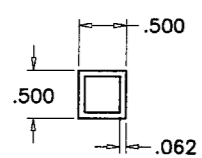
4A GLAZING TUBE
