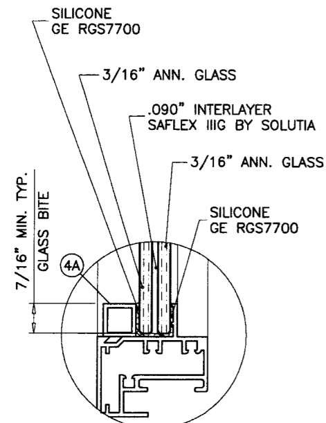
GLASS TYPE 'E'
