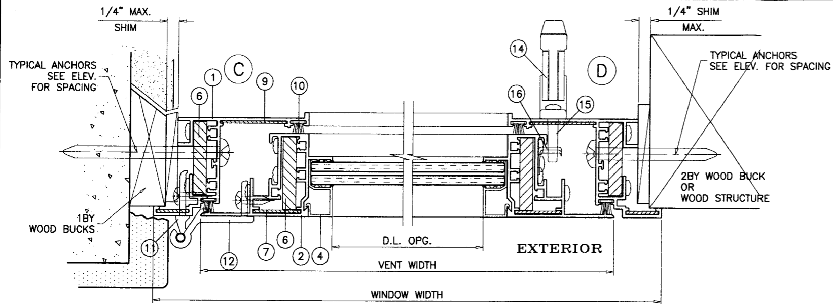
SINGLE VENT WINDOWS (BUTT HINGE OPTION)
