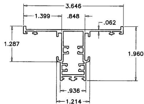
3 IMPOST
