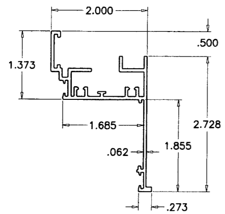
1 FRAME
