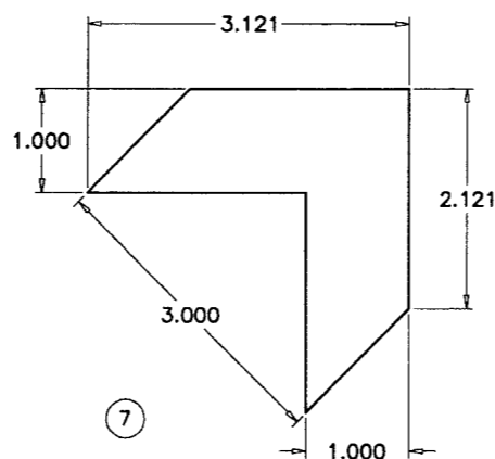
CORNER KEYS
