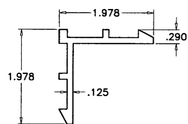
6 CORNER KEY
