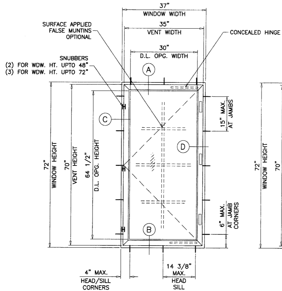
SINGLE VENT WDW.
